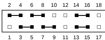
J2 - BANK 1
