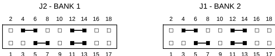
8K x 8 or 16K x 8 ROM/PROM/EPROM
