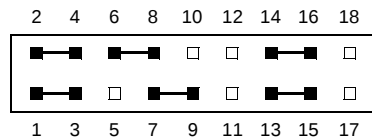
J1 - BANK 2
