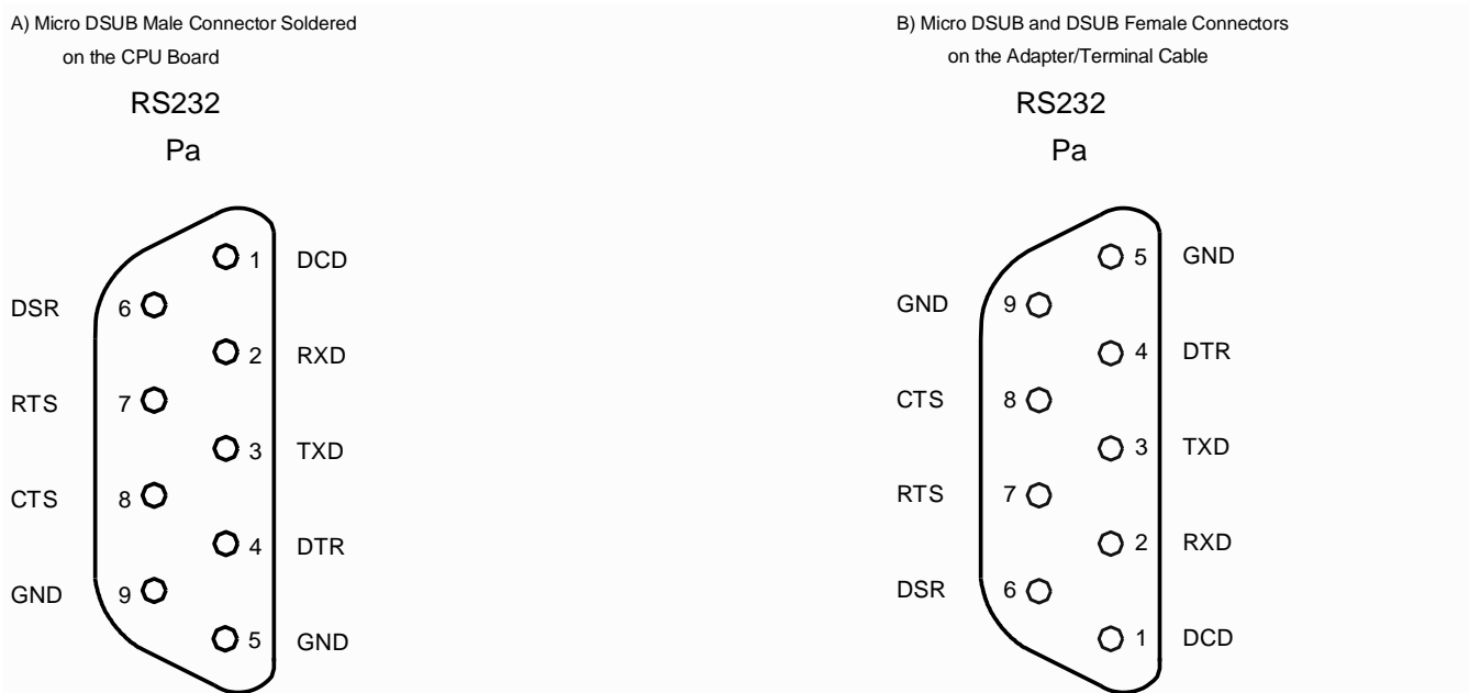
Figure 1-2: Pinout of the Micro D-Sub and D-Sub Connector for RS232
