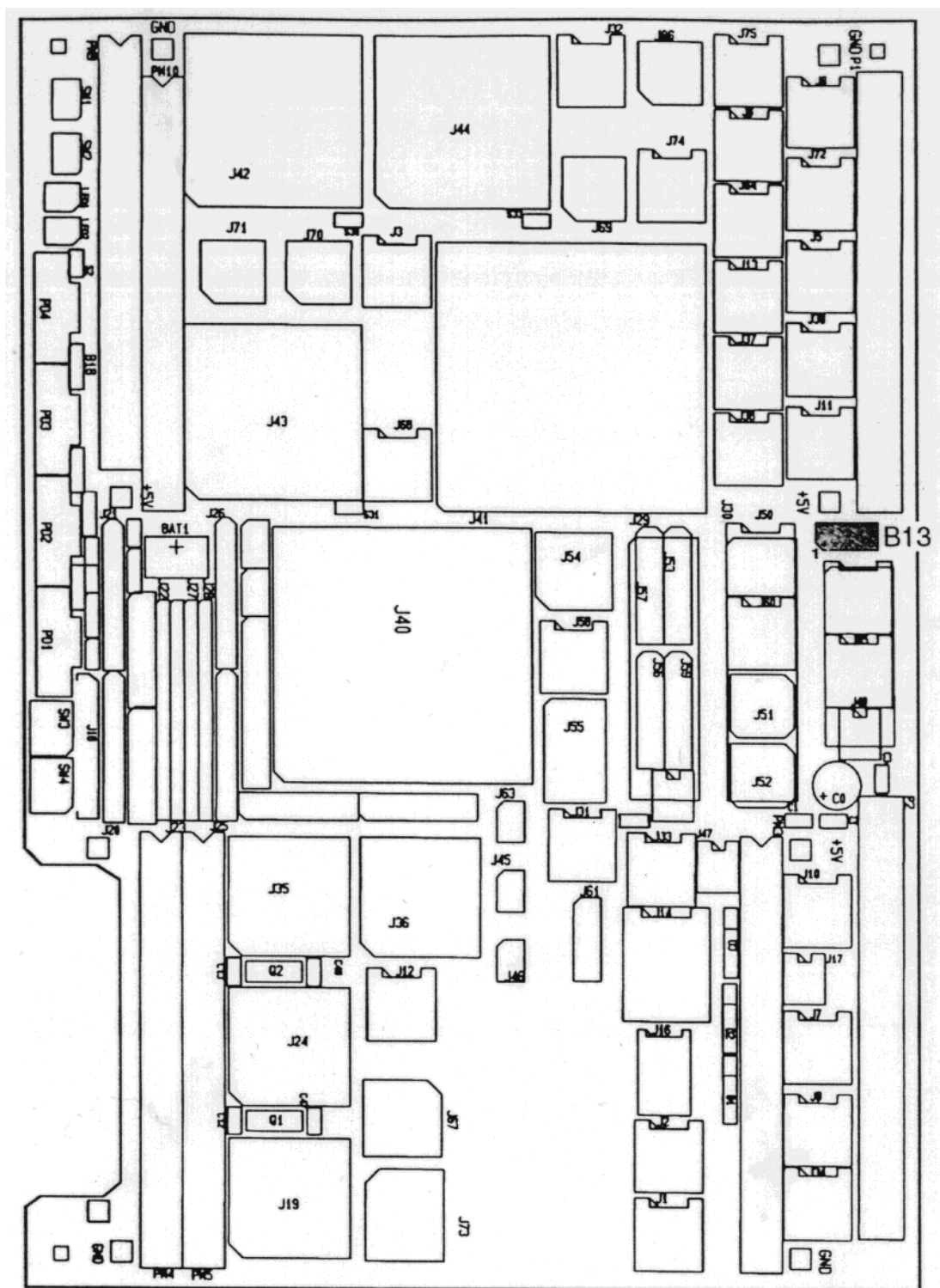
Figure 6-9: Location Diagram of Jumperfield B13
