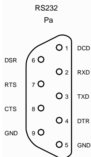
A) Micro DSUB Male Connector Soldered on the CPU Board
