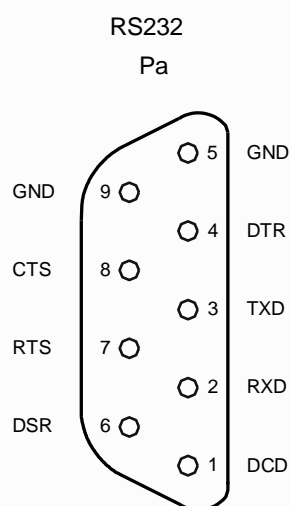
B) Micro DSUB and DSUB Female Connectors on the Adapter/Terminal Cable
